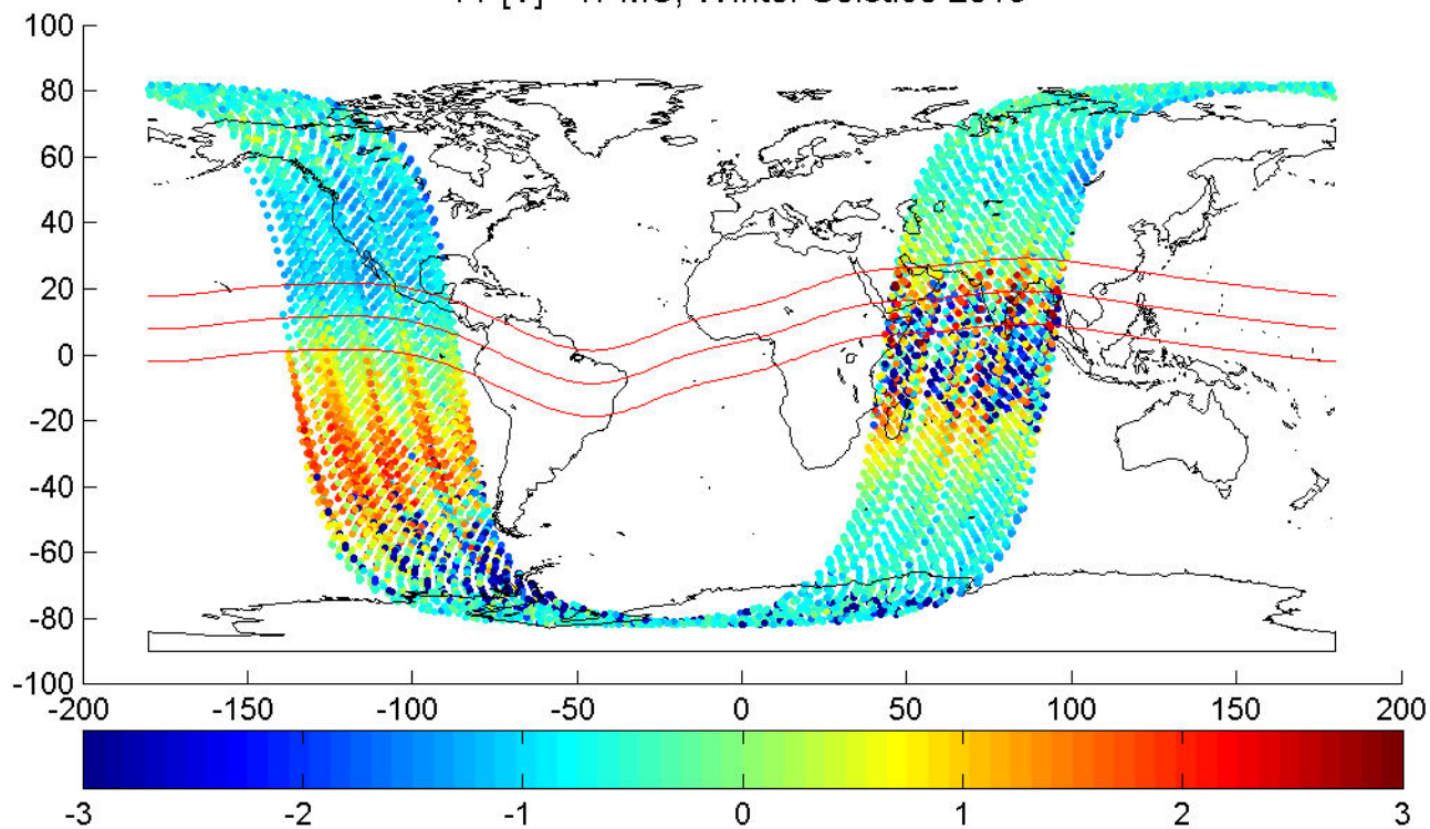
FP[V] - TPMU, Winter Solstice 2013
